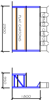
PACKING BENCHES
